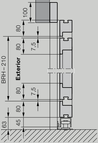
Sliding door ST 500 with wicket door
