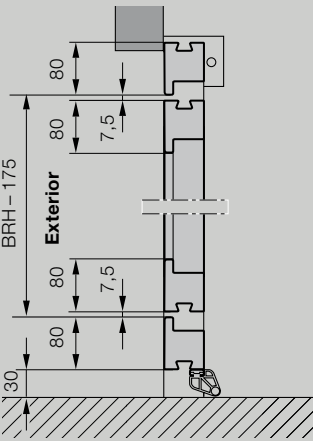
Non-protruding up-and-over door ET 500 with wicket door
